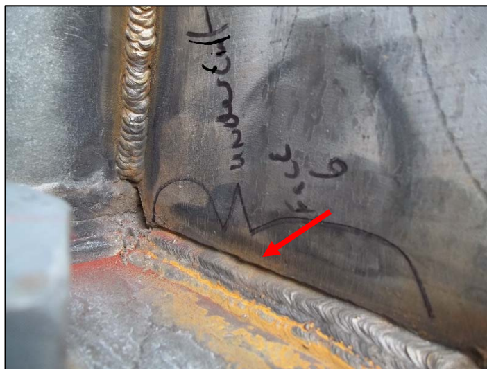
Monopole Base Plate Stiffener Underfill
