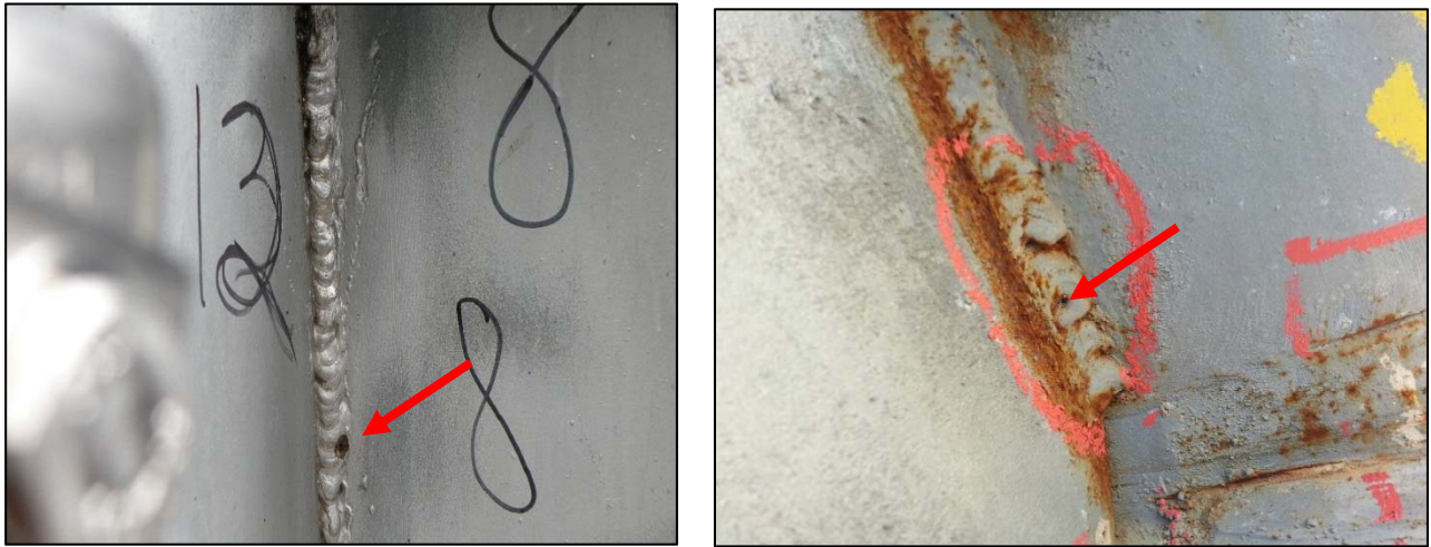
Examples of Porosity in Monopole Modification Welding
