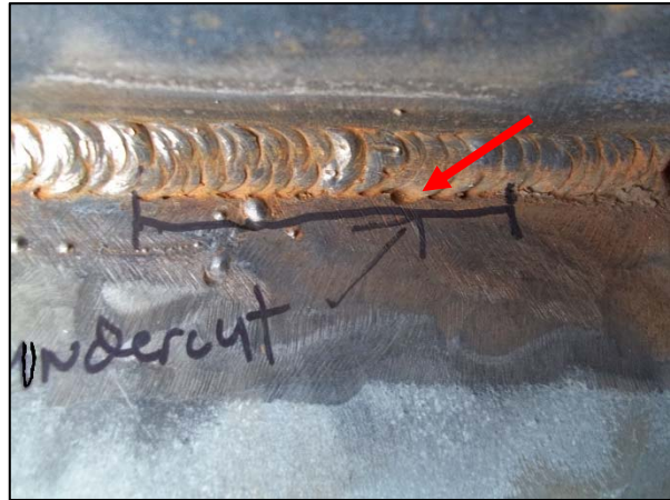
Monopole Modification Weld Undercut
