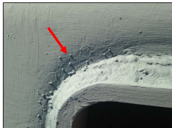
Weld Spatter at a Modification Stiffener and Field-Welded Port Installation
